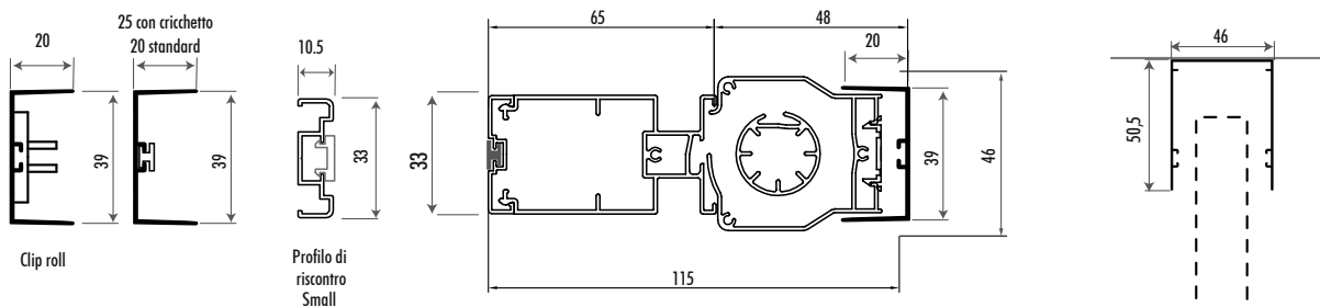
Laterale RollOut Magnum
