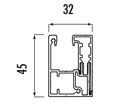
Guida laterale Side rail
